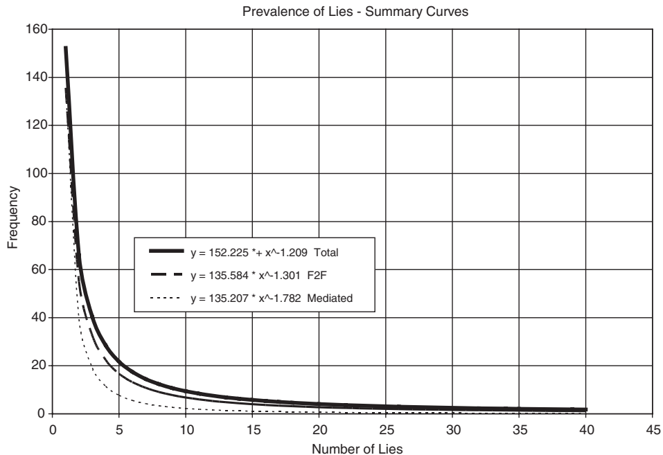
Figure 4 Frequencies of total, face-to-face, and mediated lies are represented by similar standard power functions.
