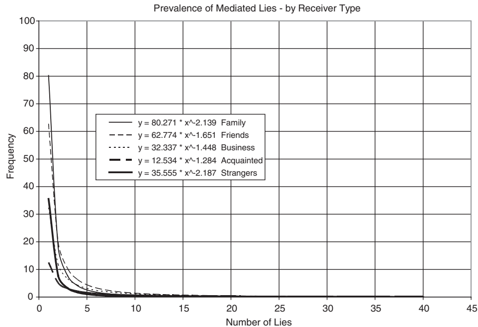
Figure 6 Standard power function curves fit the frequencies of mediated lies plotted by number of lies for all receiver types.
